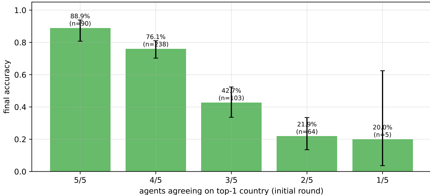
Agreement vs. accuracy
